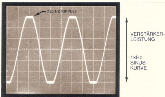
HARD CLIPPING (Abb. 3)
