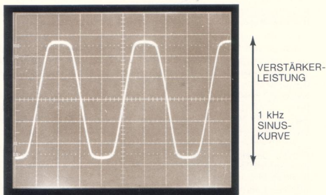
SOFT CLIPPING (Abb. 4)
