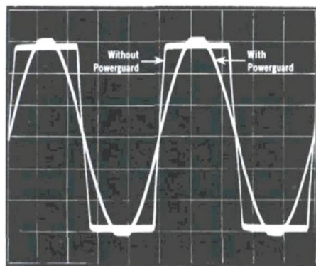
Oscilloscope of output waveform with and without Power Guard. Input overdriven for each trace 20 dB.
