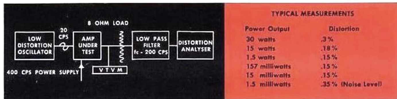
Test set up to measure distortion at very low power
