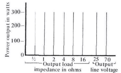
Fig. 6 - Performance of MC 2300
