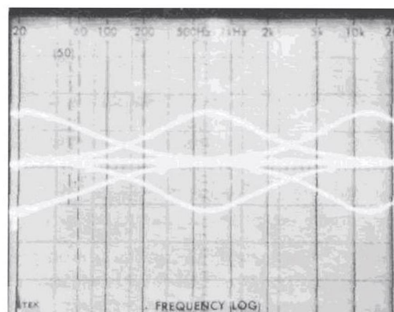
Fig. 9—Range of equalizer controls, McIntosh MX 117 Tuner-Preamp
