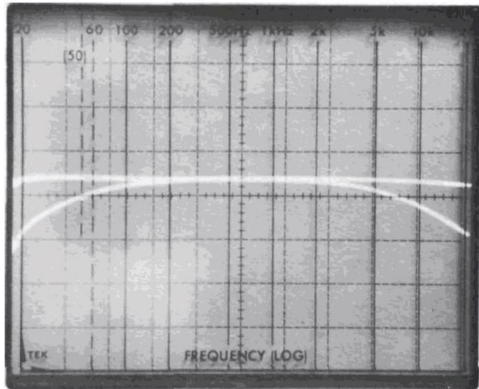
Fig. 7 - Low-cut and high-cut filter response
