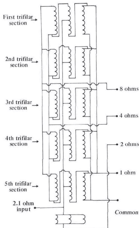
Fig. 9 - MC 2205 output auto-transformer schematic diagram
