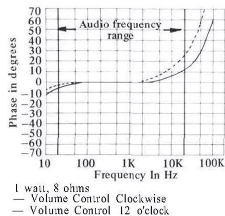
Fig. 8B - Typical phase shift in a complete McIntosh amplifier
