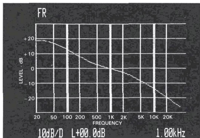
Fig. 11—Phono preamp-equalizer response, McIntosh MX 117 Tuner-Preamp
