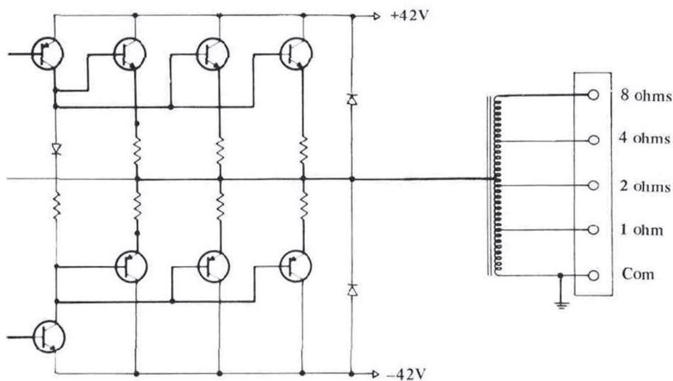
Fig. 5 - McIntosh MC 2205 output stage and transformer
