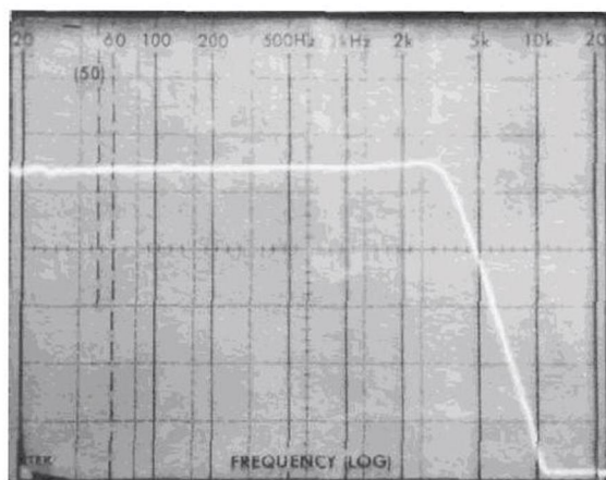
Fig. 8—Frequency response, AM section, McIntosh MX 117 Tuner-Preamp
