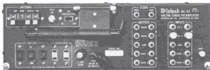
Fig. 2—Rear panel view of McIntosh MX 117 Tuner-Preamplifier
