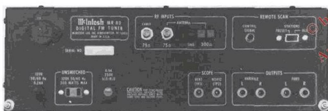
Fig. 2 Rear Panel view of McIntosh MR 80 Tuner.
