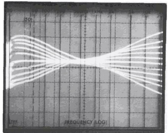
Fig. 6 - Step-by-step tone control response characteristics
