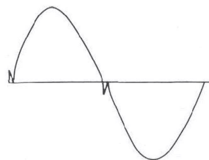
Fig. 2 - Notch distortion in a typical Class B output circuit
