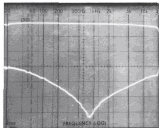
Fig. 6—Frequency response (upper trace) and stereo separation, McIntosh MX 117 Tuner-Preamp
