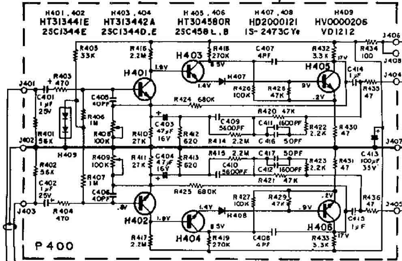
Marantz - 4400 P-400 Phono Preamp
