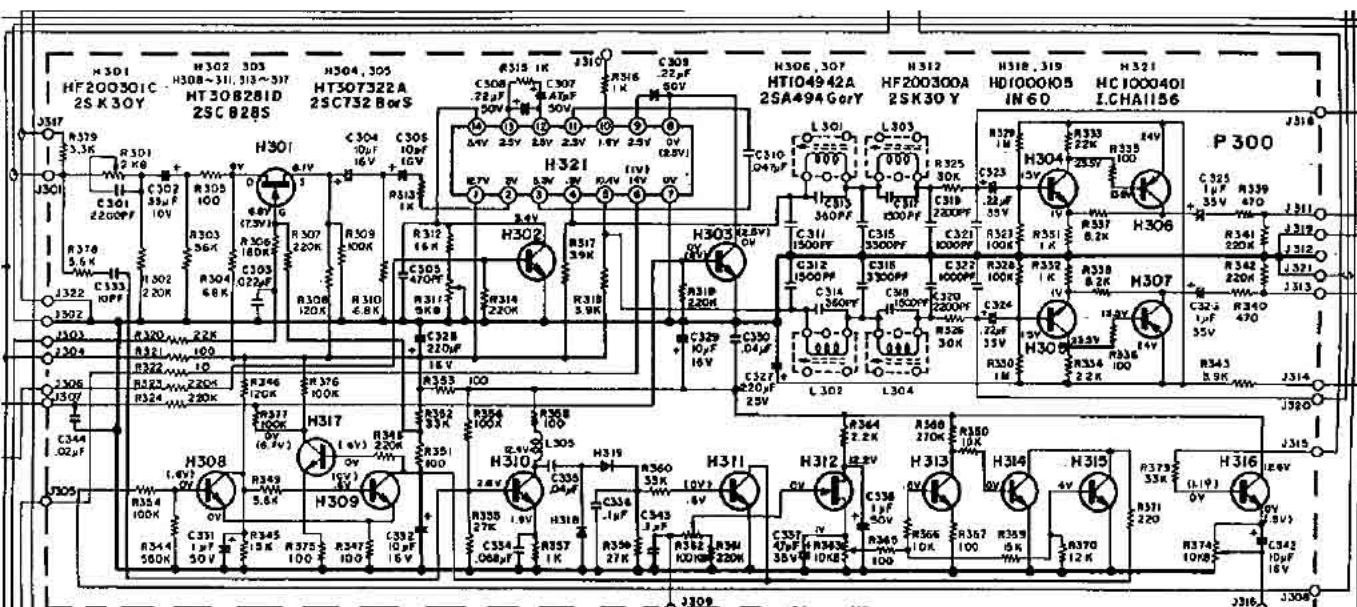
Marantz - 4400 P-300 FM Multiplex PLL
