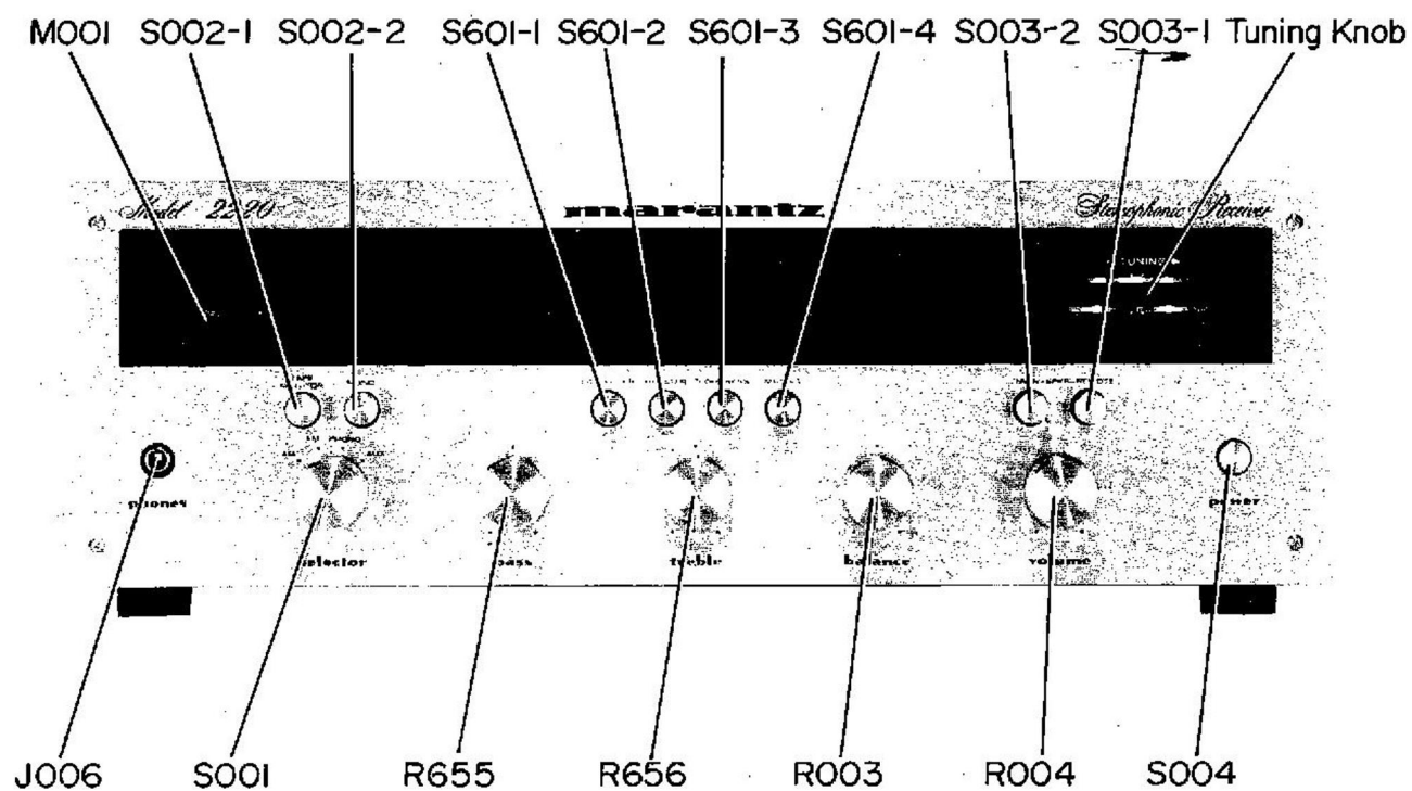
Figure 2. Front Panel Adjustments and Component Locations
