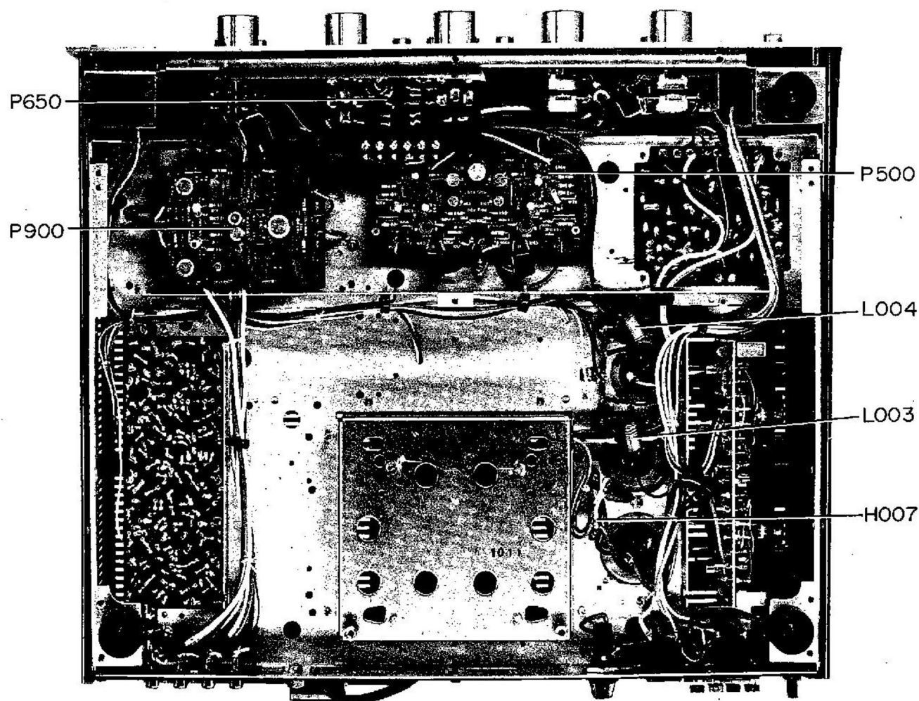
Figure 5. Main Chassis Component Locations (Bottom View)
