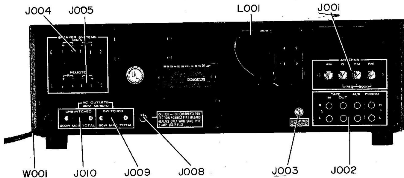
Figure 4. Rear Panel Adjustment and Component Locations
