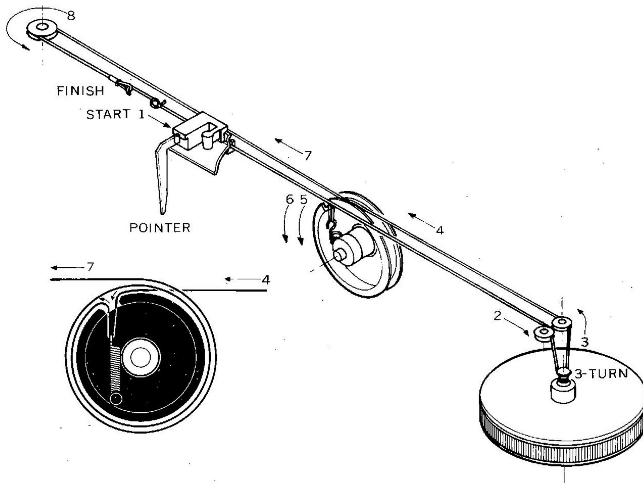
Figure 1. Dial Stringing
