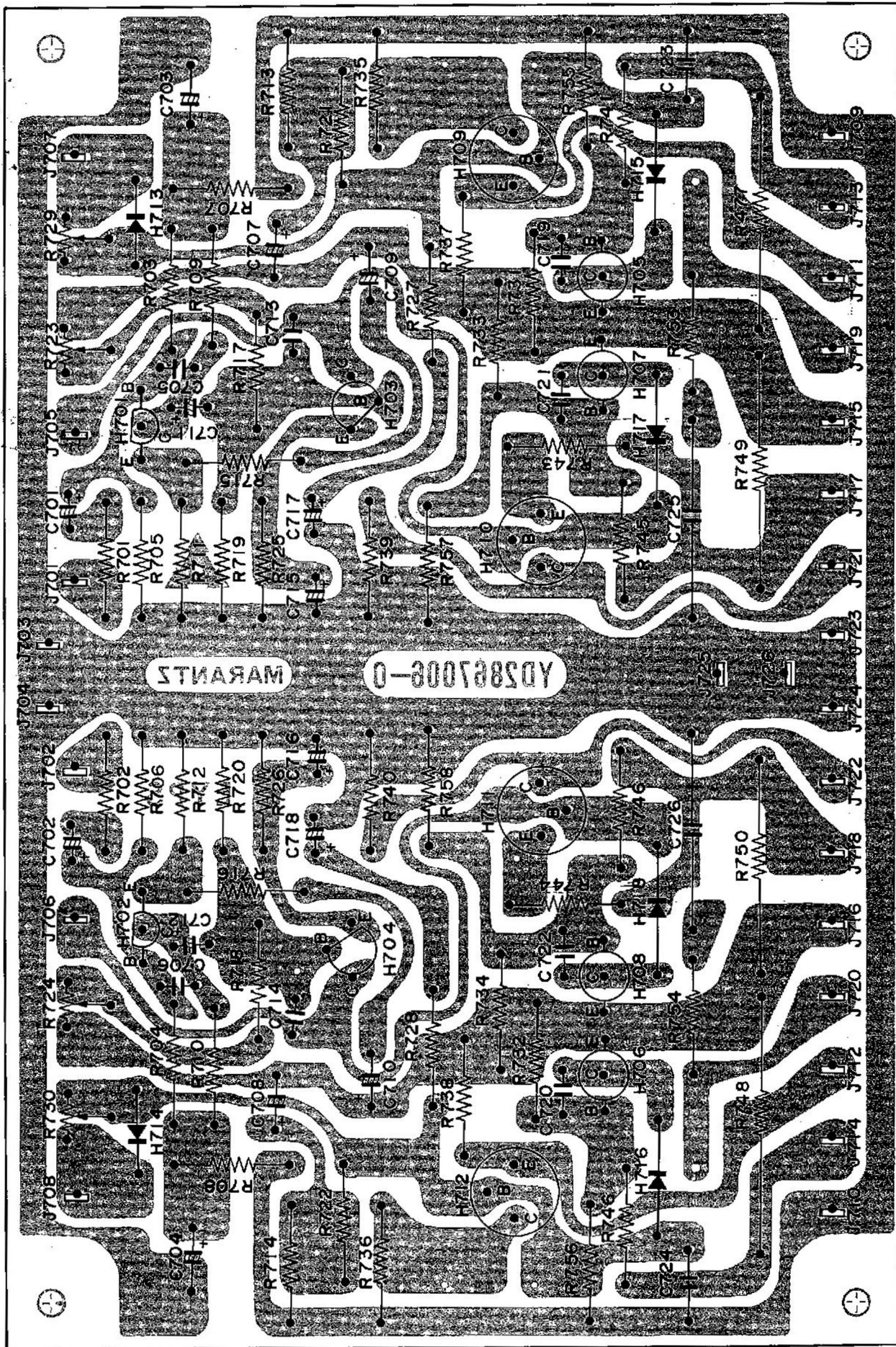
Figure 12. Power Amplifier Assembly P700 Component Locations
