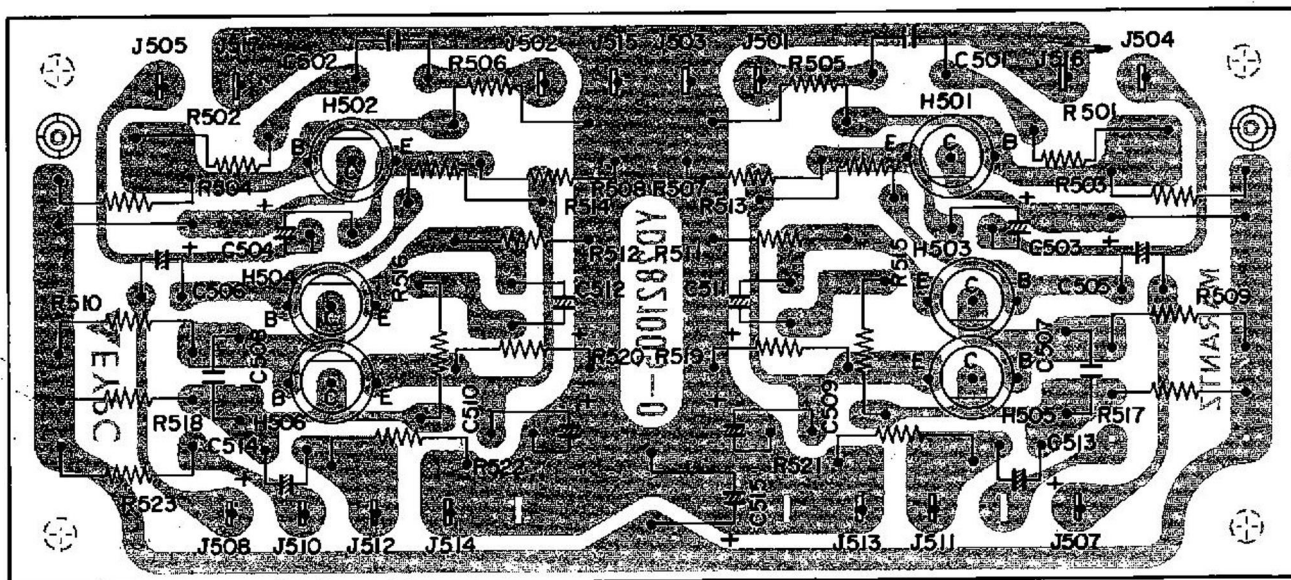
Figure 10. Tone Amplifier Assembly P500 Component Locations
