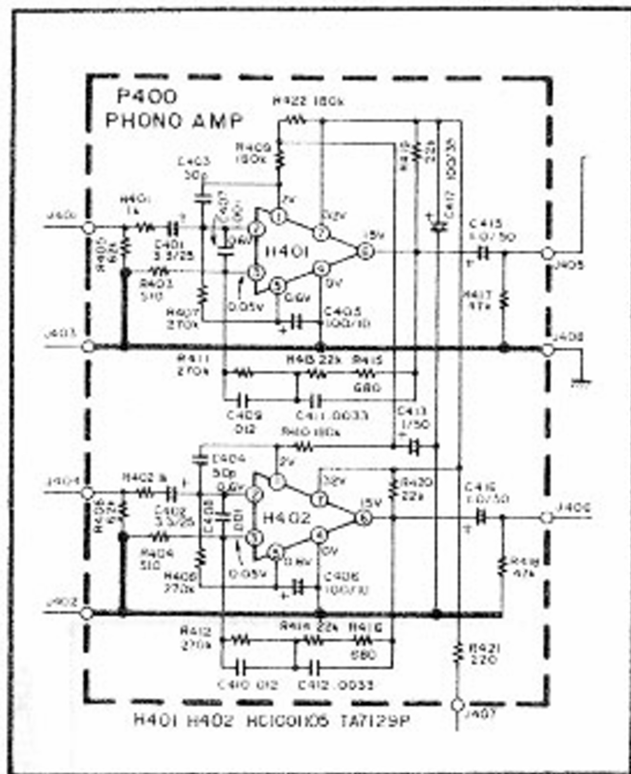
Phono Amplifier Assembly (P400) Schematic Diagram
