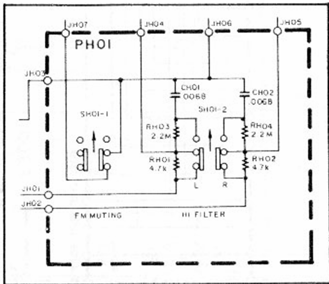
Figure 20 Muting Hi Filter Assembly (PH01) Schematic Diagram
