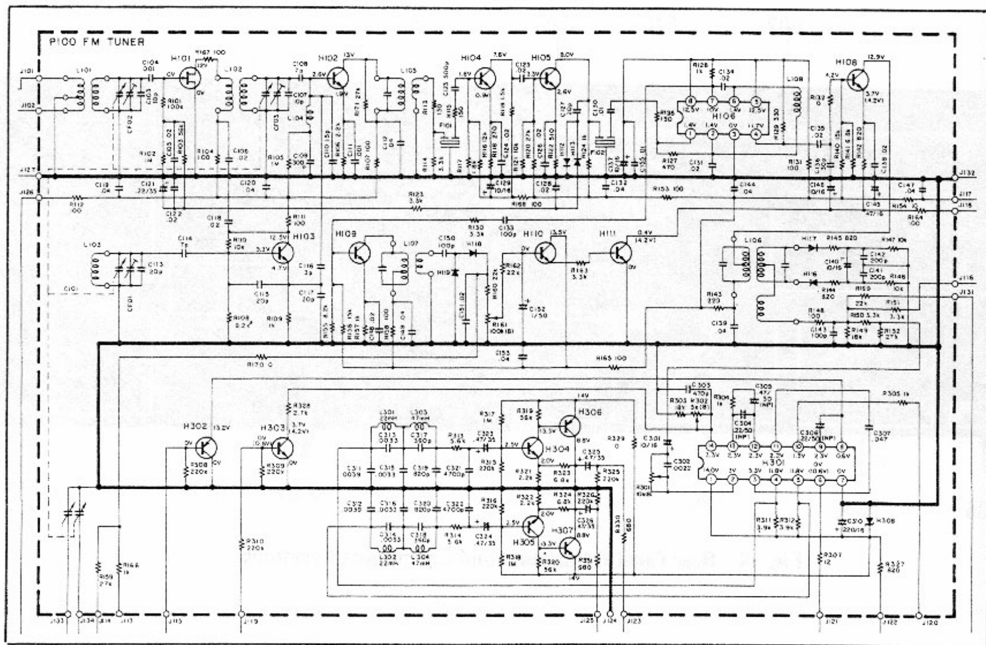
Fig. 6 FM Tuner Assembly (P100) Schematic Diagram
