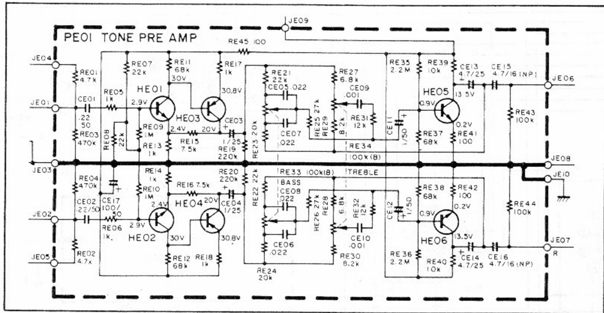
Figure 18 Tone Amplifier (PE01) Schematic Diagram
