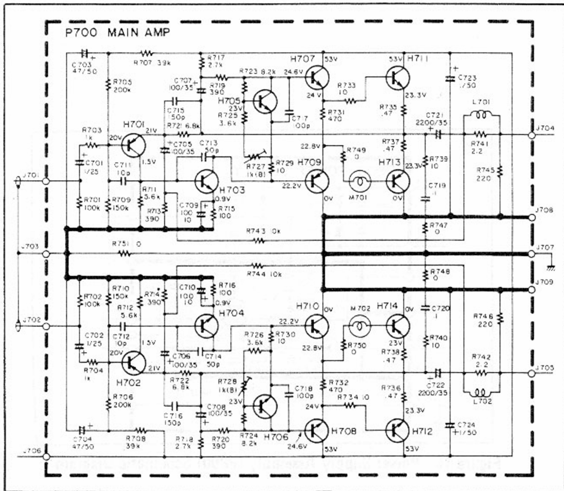
Figure 14 Power Amplifier Assembly (P700) Schematic Diagram
