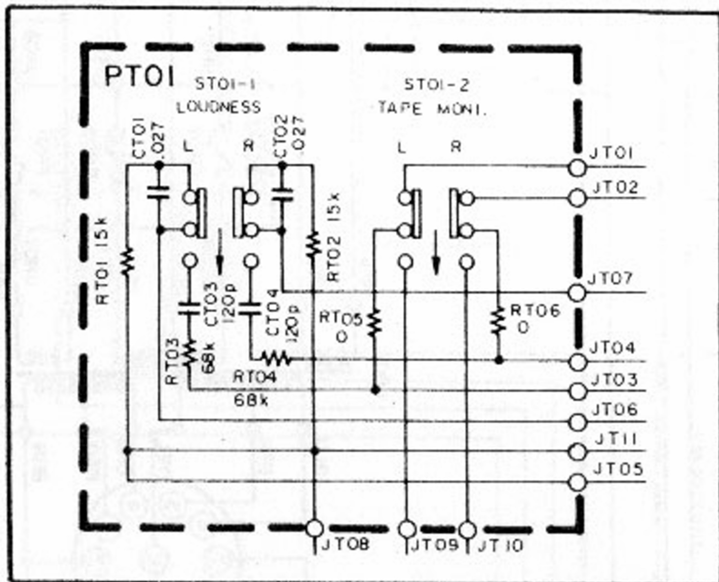
Figure 22 Loudness and Monitor Assembly (PT01) Schematic Diagram
