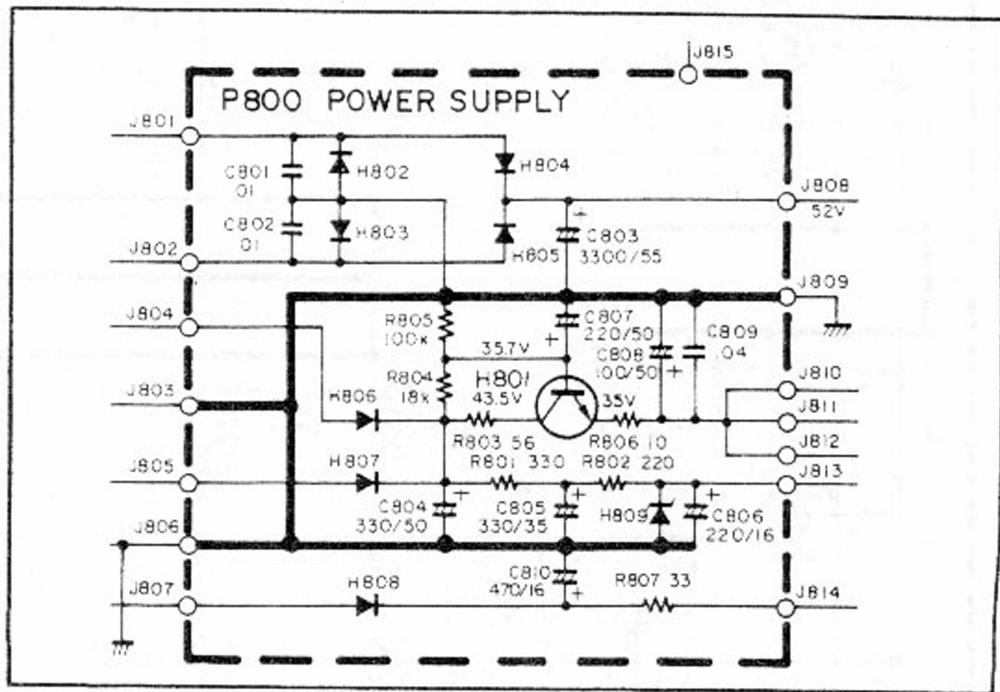
Figure 16 Power Supply Assembly (P800) Schematic Diagram
