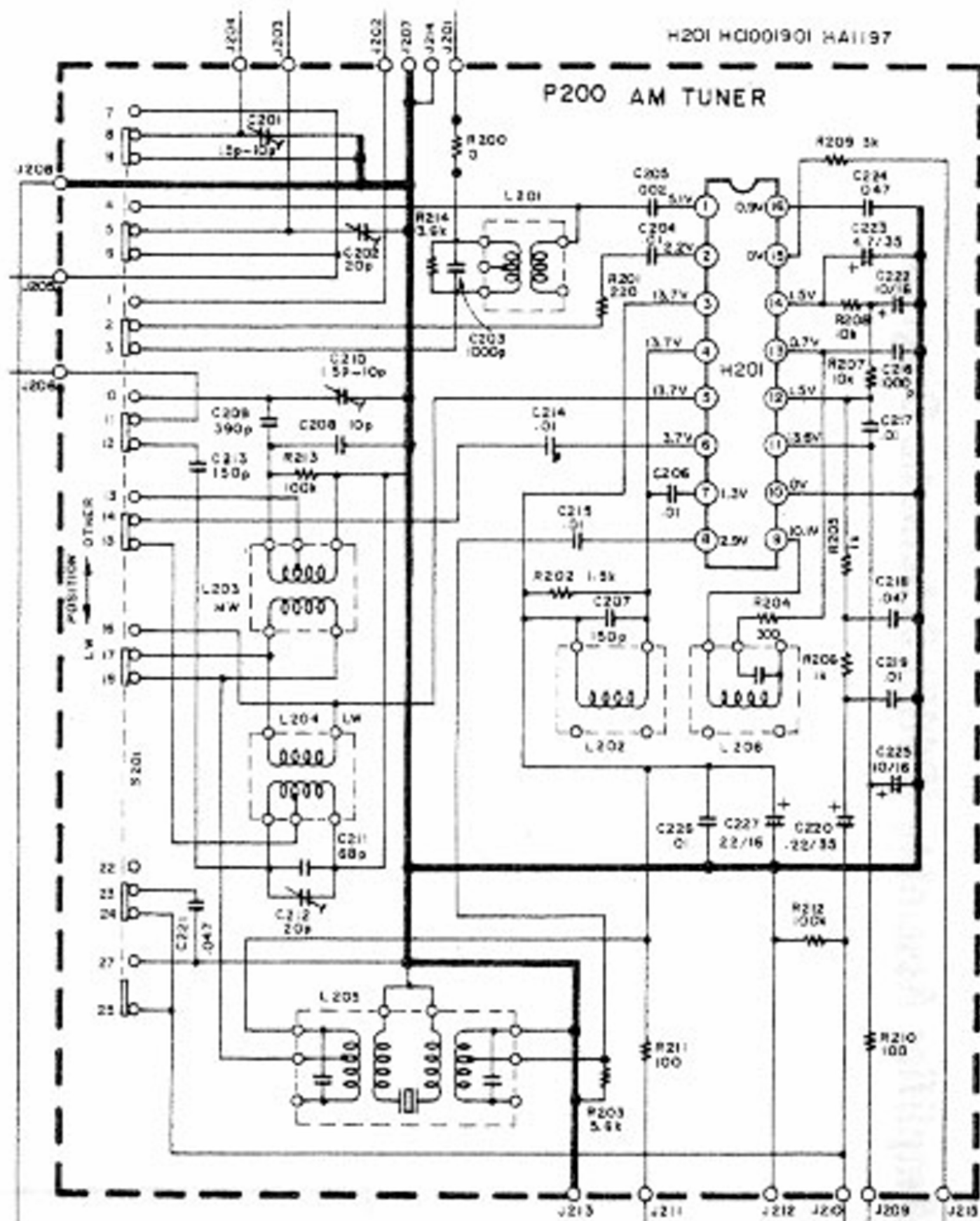
Fig. 8 AM Tuner Assembly (P200) Schematic Diagram
