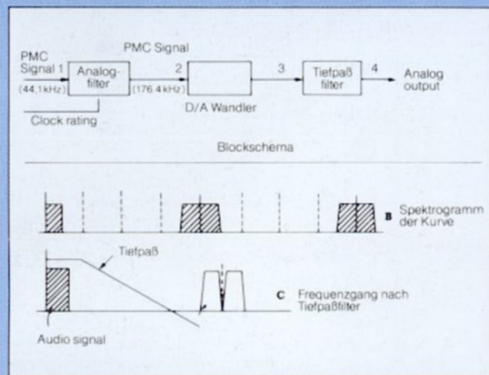
Schema Z-Filter
