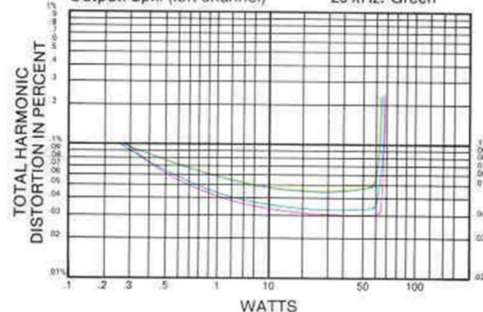
MODEL: 2250B Input: Aux (both channels) Output: Spkr (left channel) 20 Hz: Blue 1 kHz: Red 20 kHz: Green
