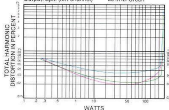
MODEL: 2325 Input: Aux (both channels) Output: Spkr (left channel) 20 Hz: Blue 1 kHz: Red 20 kHz: Green
