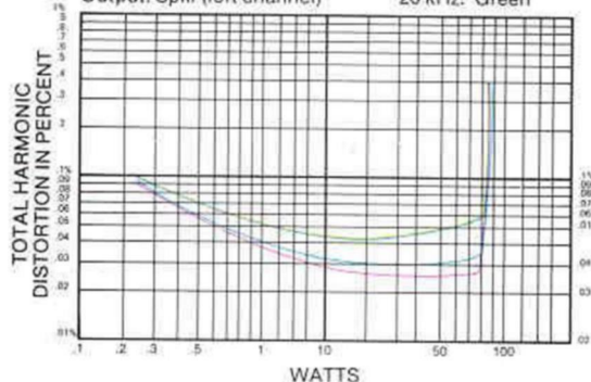
MODEL: 2275 Input: Aux (both channels) Output: Spkr (left channel) 20 Hz: Blue 1 kHz: Red 20 kHz: Green
