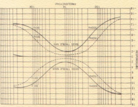
TONE CONTROL
