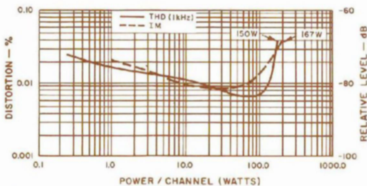
Fig. 6 — Distortion vs. power output.
