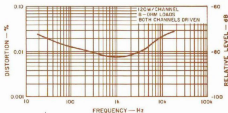
Fig. 7 — Distortion vs. frequency at rated output.
