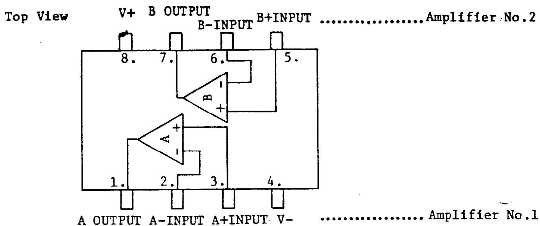
Equivalent Circuit (1/2)
