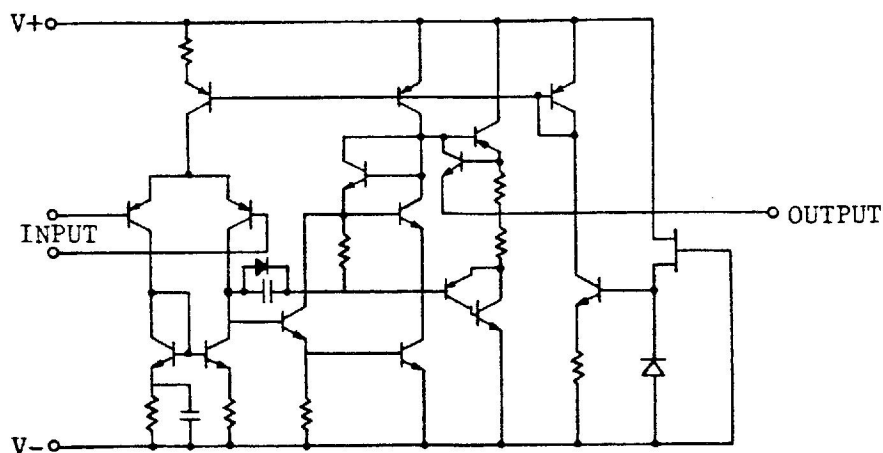
Equivalent Circuit (1/2)
