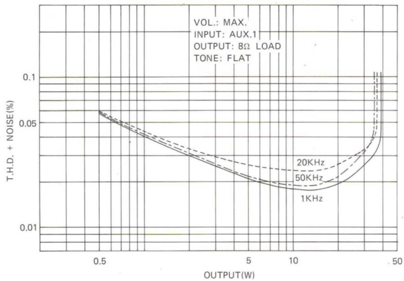
POWER T.H.D. (BOTH CH. DRIVEN)
