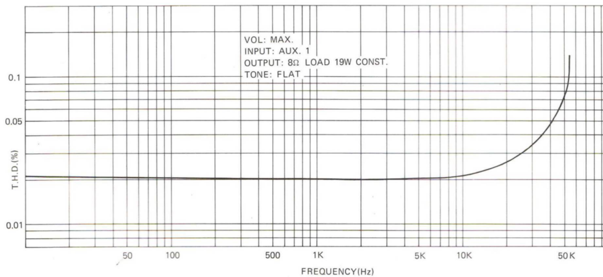
FREQUENCY T.H.D. (BOTH CH. DRIVEN)
