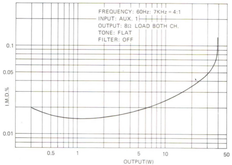
POWER I.M.D. (BOTH CH. DRIVEN)
