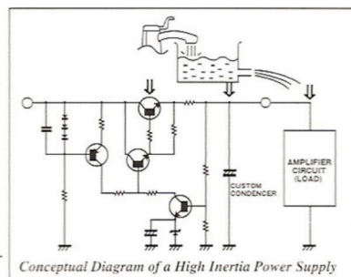
Conceptual Diagram of a High Inertia Power Supply
