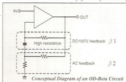
Conceptual Diagram of an OD-Beta Circuit
