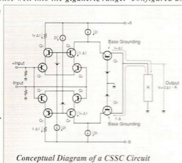
Conceptual Diagram of a CSSC Circuit
