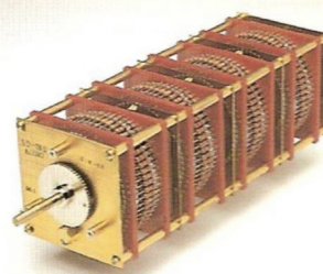
Ultimate Volume (C-9) 4-ganged Super Ultimate Attenuator (C-10)
