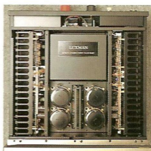
Large-Capacitance Power Transformer, Capacitors and Heat Sinks (C-10)
