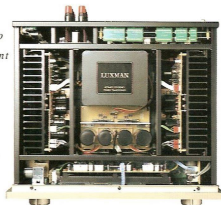
Internal Shielding Construction (L-503s)
