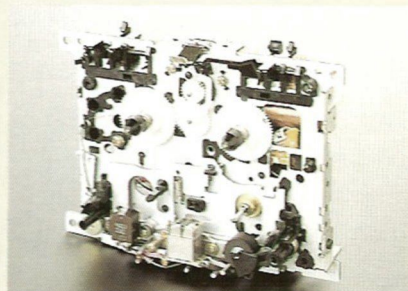
Diecast Aluminium Base
