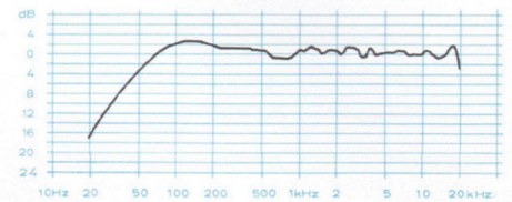
Frequenzgang OY
