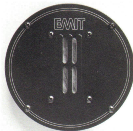
Rotatable Electromagnetic Induction Tweeter. Its etched voice-coil on a planar diaphragm is driven by magnets of rare-earth samarium cobalt, six times stronger than ferrite.
