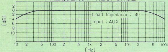
FREQUENCY RESPONSE
