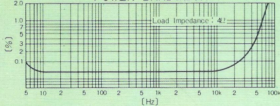
POWER BANDWIDTH
