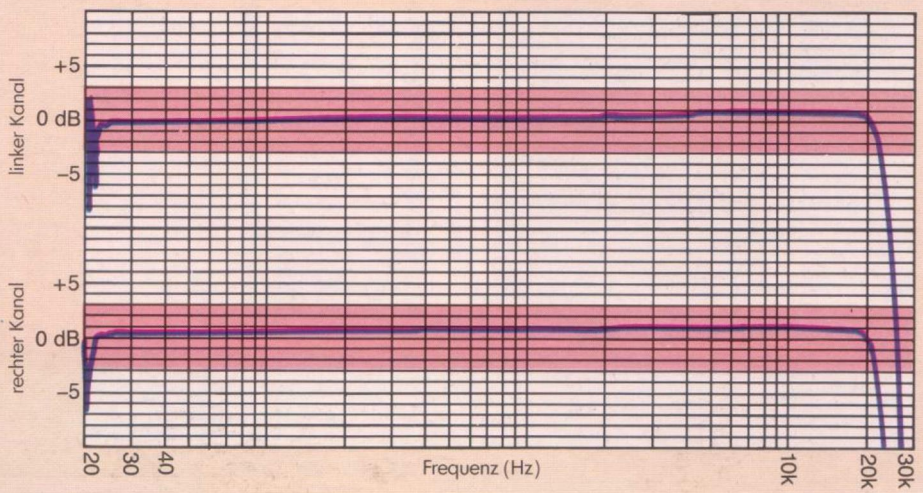
FREQUENZGANG
