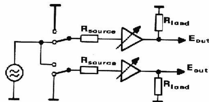
Fig. 4: Test set-up to measure crosstalk
