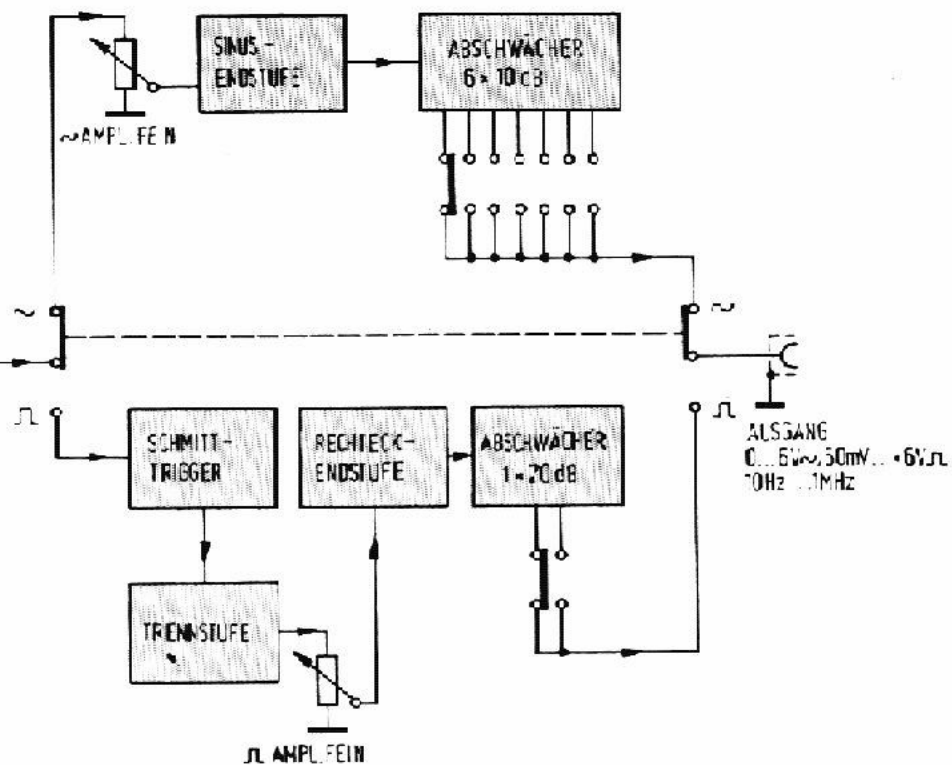
Fig. 1: Block schematic diagram
