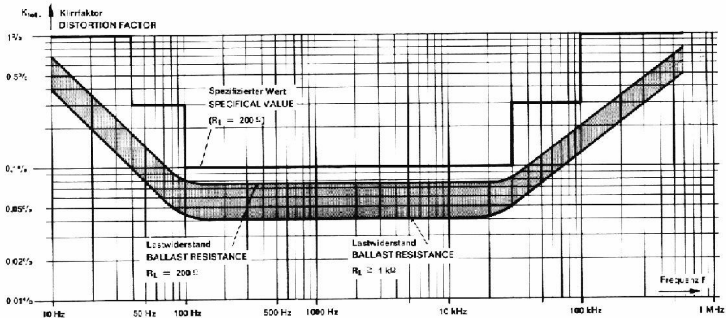
Fig. 5: Typical curve of the distortion factor at maximum output voltage
