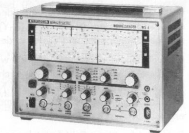
Wobbelsender WS 4 Wobbulator WS 4
