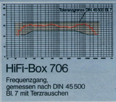
GRUNDIG HiFi-Box 706 Compact -70 Watt
