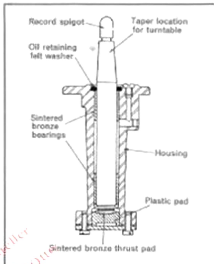
Figure 2. Section of turntable spindle bearing assembly
