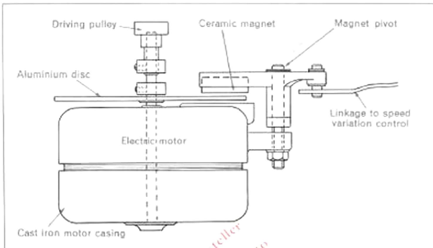
Figure 3. Eddy current brake for speed regulation
