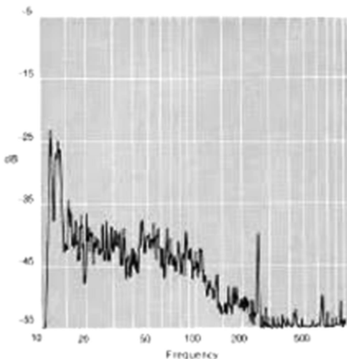
Figure 5. Typical curve showing rumble levels
