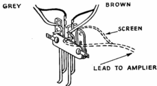
Connections for Monophonic Pickups Diagram Three
