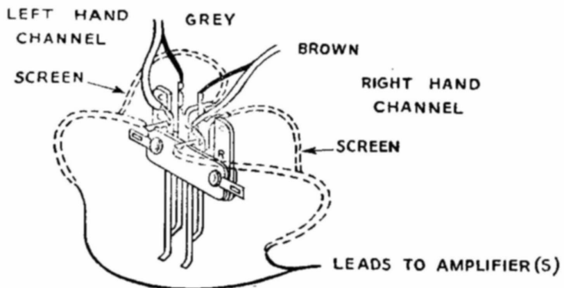
Connections for Stereophonic Pickups Diagram Four
