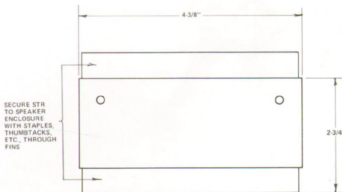
FIGURE 1 – Dimensions
