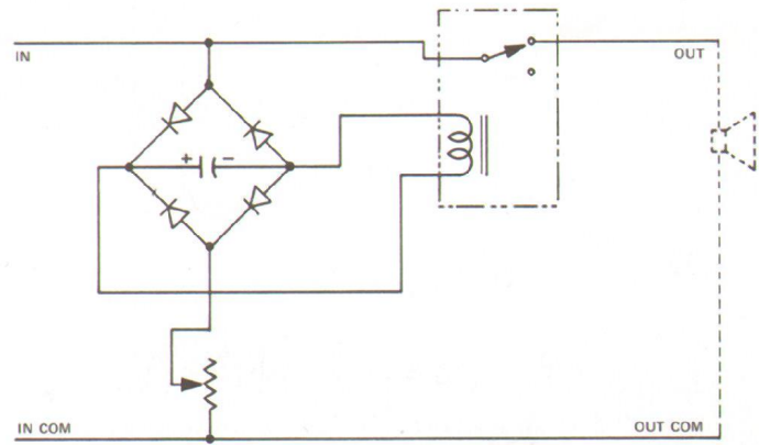
FIGURE 2 — Wiring Diagram
