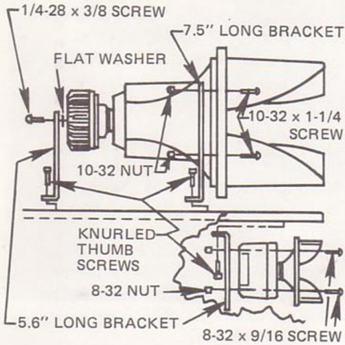
FIGURE 3 – Bracket Assembly
