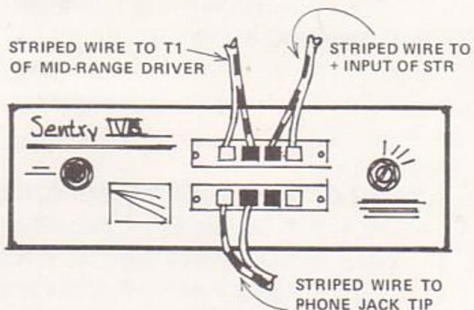
FIGURE 5 – Crossover Wiring
