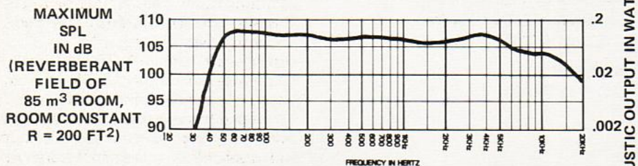
FIGURE 5- Maximum Acoustic Output
