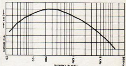
FIGURE 7 — Random Noise Spectrum Specified by D.I.N. 45573 for Power Testing of Loudspeakers (1/10 Octave Analyzer)
