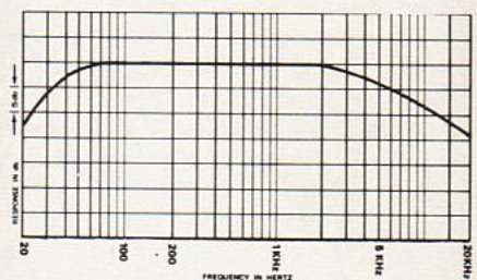
FIGURE 9 — Random Noise Spectrum for Testing Sentry 100A (1/10 Octave Analyzer)
