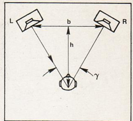
FIGURE 6 — Speaker/Listener Location for Good Stereo Imaging
