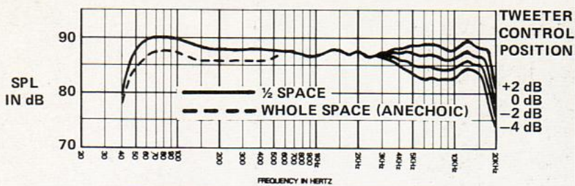
FIGURE 1 - Axial Frequency Response 2 Volts/3 Feet
