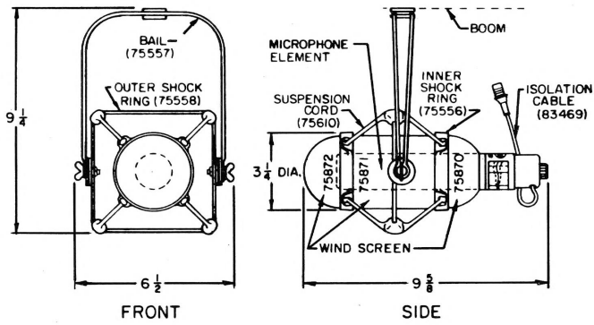
Figure 3 - Dimensions
