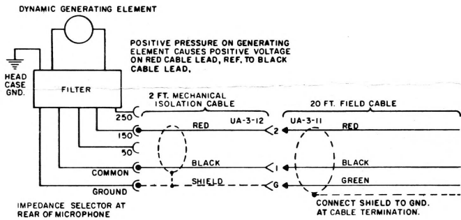
Figure 4 - Wiring Diagram
