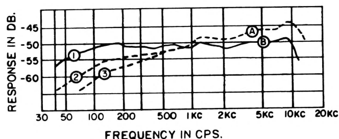
Figure 1 - Frequency Response
