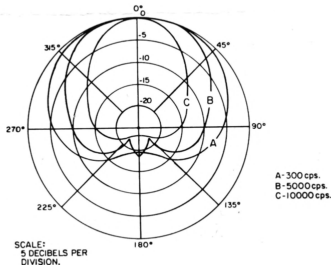
Figure 2 - Polar Pattern
