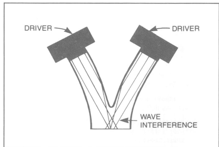
FIGURE 2 "Y" Manifold Showing Ray Interferences
