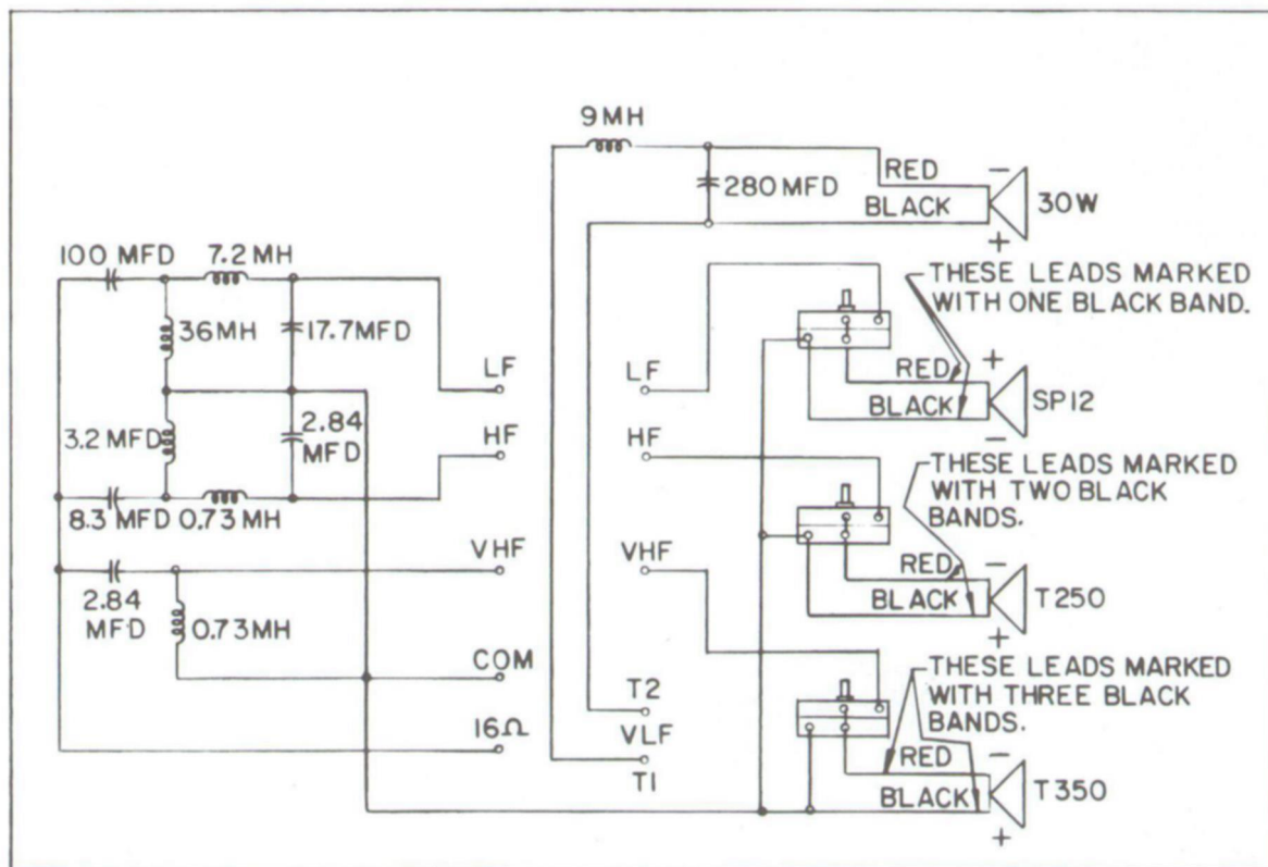
FIGURE 2 - Schematic Wiring Diagram
