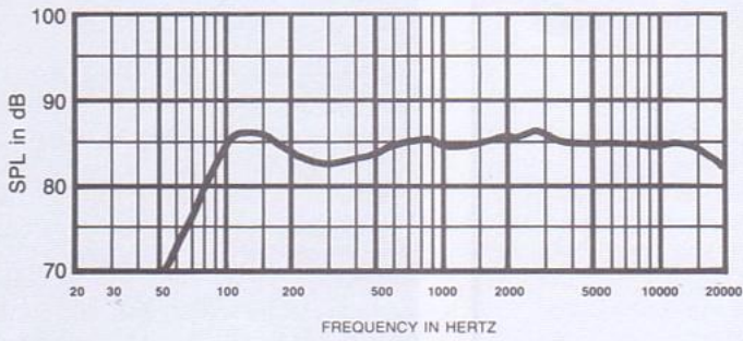
FIGURE — 1 Axial Frequency Response
