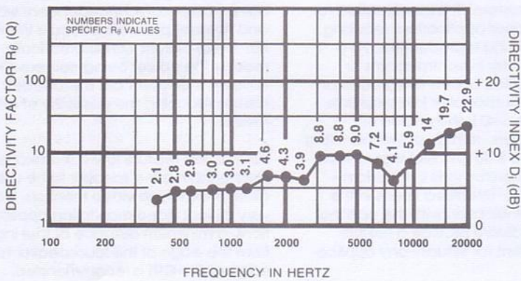
FIGURE — 3 Directivity vs. Frequency Whole Space (anechoic)
