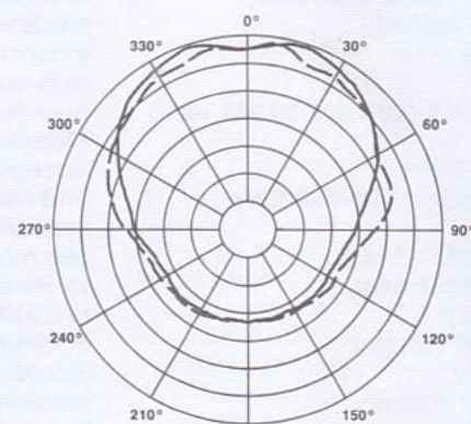
FIGURE — 4 Polar Response
