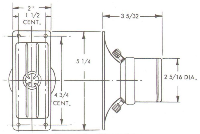
Figure 1 - Dimensions
