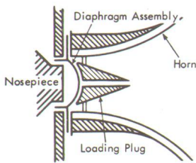
Figure 2 Sonophase drawing
