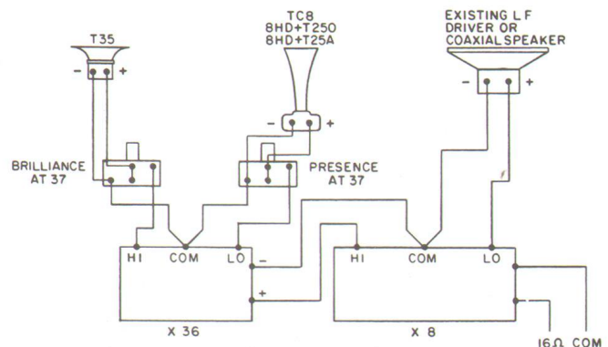
Figure 5B - Three-way system drawing
