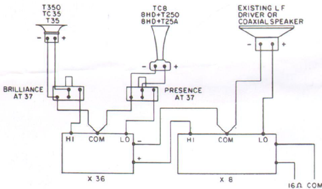
Figure 5B - Three-way system drawing
