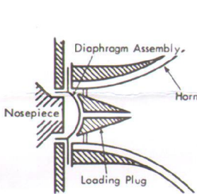
Figure 2 Sonophase drawing
