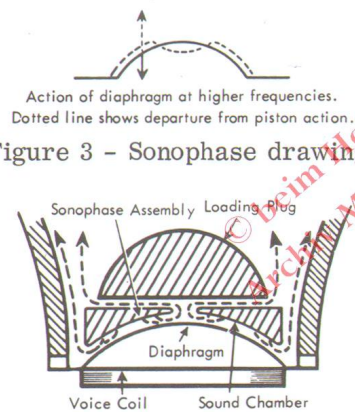
Figure 3 - Sonophase drawing
