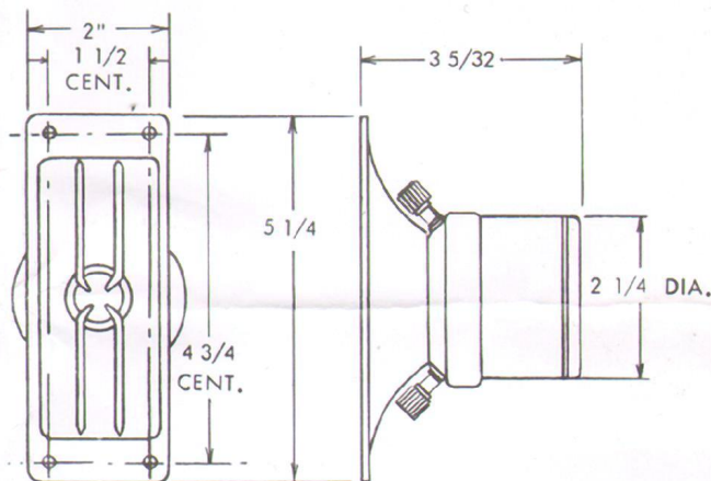
Figure 1 - Dimensions
