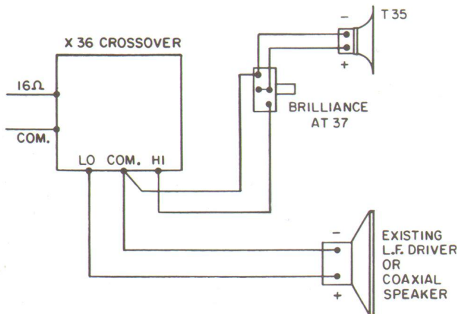
Figure 5A - Two-way system wiring
