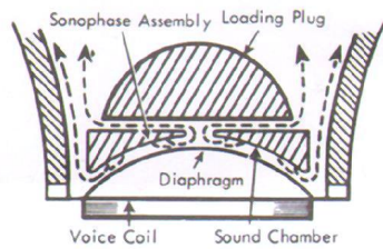
Figure 4 - Sonophase drawing
