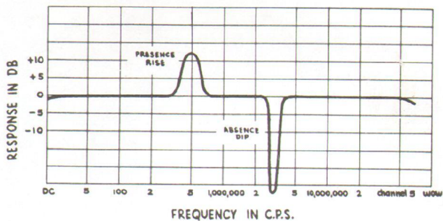
Fig. 3 — Frequency Response at 791-watt Level
