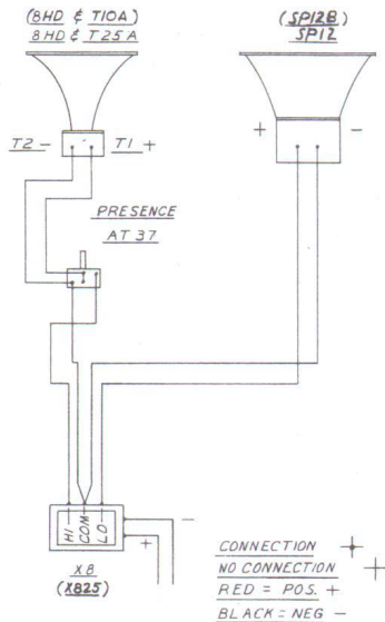
Fig. 2 — Schematic Wiring Diagram Separate 2-way System
