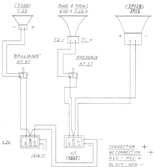
Fig. 3 — Schematic Wiring Diagram Separate 3-way System
