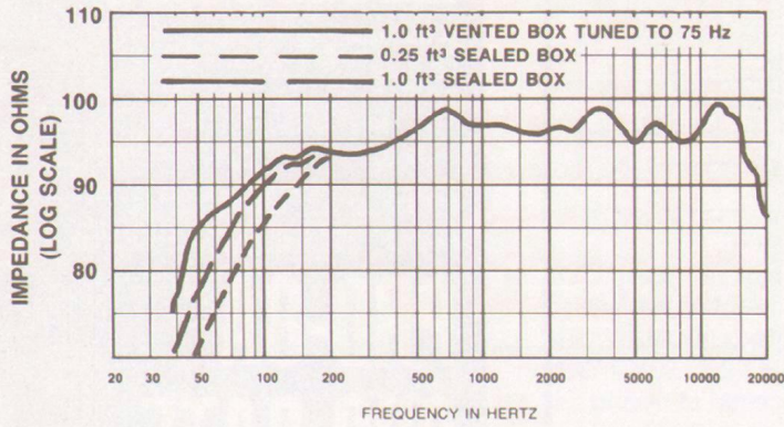
FIGURE 1 — Axial Frequency Response 1 Watt/1 Meter
