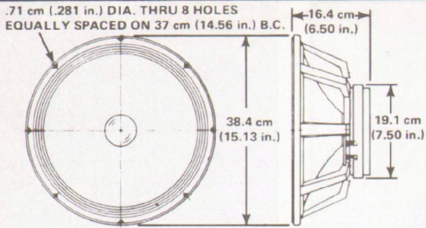
FIGURE 1 - Dimensions
