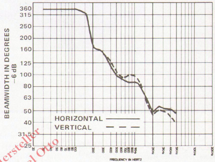
FIGURE 4 TL606/EVM.15B Beamwidth vs. Frequency
