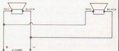
FIGURE 11 Connection of 2 EVM .15B Speakers in Parallel
