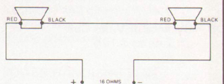
FIGURE 12 Connection of 2 EVM .15B Speakers in Series
