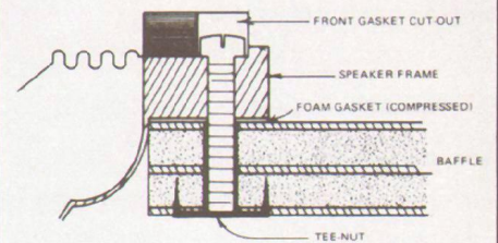
FIGURE 9 Front Mounting Detail (Not to scale)
