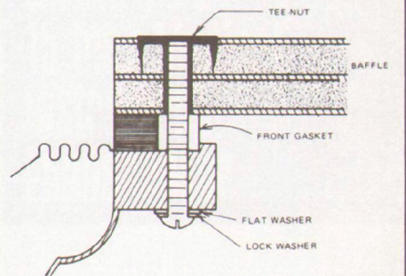
FIGURE 10 Rear Mounting Detail (Not to scale)
