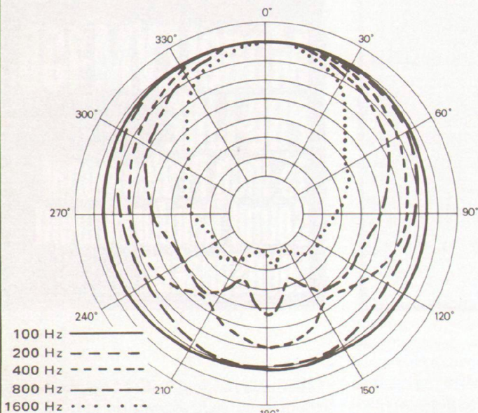
FIGURE 3 – TL606/EVM.15B Polar Response 4 V RMS of Octave Band Limited Pink Noise in Anechoic Environment, 10 ft on axis in Horizontal Plane (5 dB per Division)
