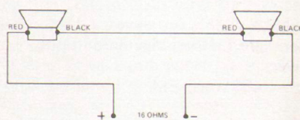
FIGURE 12 Connection of 2 EVM-15B Speakers in Series
