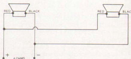
FIGURE 11 Connection of 2 EVM-15B Speakers in Parallel
