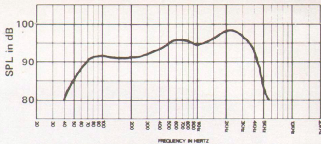
FIGURE 2 – TL606/EVM.15B Frequency Response (Swept 1/3-Octave Band Pink Noise, 4 V at 10 ft on Axis, Half-Space Environment)
