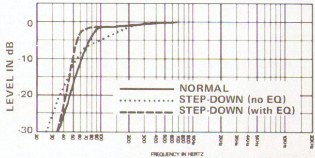
FIGURE 6 TL806/EVM .12L Low Frequency Response
