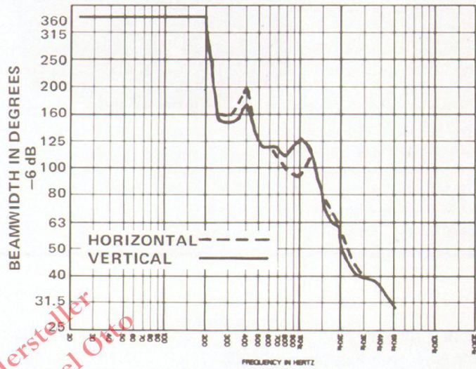
FIGURE 4 TL806/EVM .12L Beamwidth vs. Frequency
