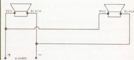
FIGURE 11 Connection of 2 EVM-12L Speakers in Parallel
