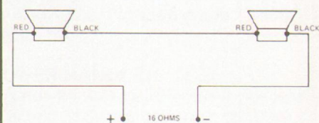
FIGURE 12 Connection of 2 EVM-12L Speakers in Series
