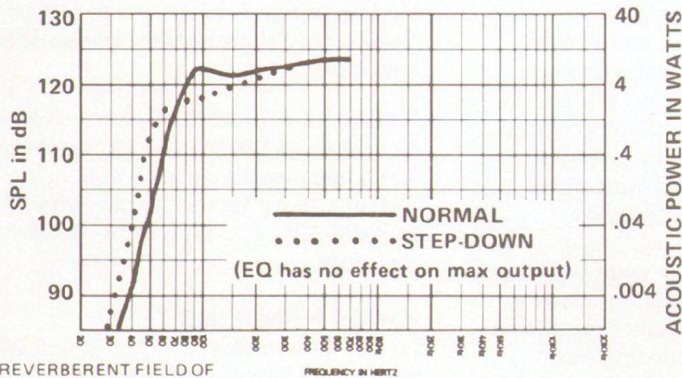
FIGURE 7 TL806/EVM .12L Theoretical Low Frequency Maximum Acoustic Output vs. Frequency
