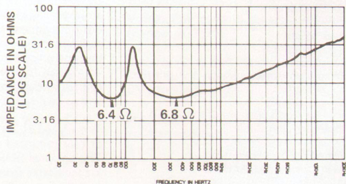
FIGURE 8 TL806/EVM .12L Input Impedance vs. Frequency
