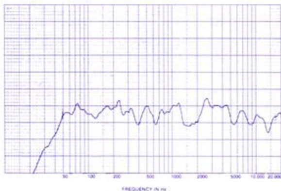
FREQUENCY RESPONSE GRAPH
