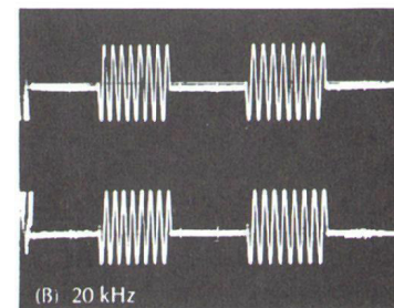
Fig. 3—Tone-burst pattern of PAT-4.
