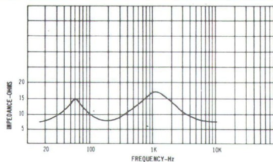
Fig. 2—Impedance characteristics.
