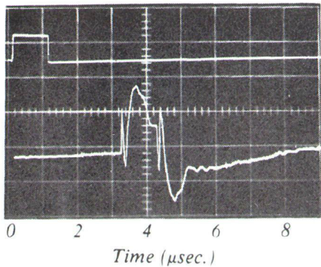
Figure 2 — Pulse Response. Upper trace: 1 msec pulse from power amplifier. Lower trace: acoustical pulse from loudspeaker.
