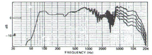
Figure 4 — Frequency response measurements on a second A-25. The family of curves represents on-axis performance with the high-frequency control at various settings. The middle curve is for the control set at "normal".
