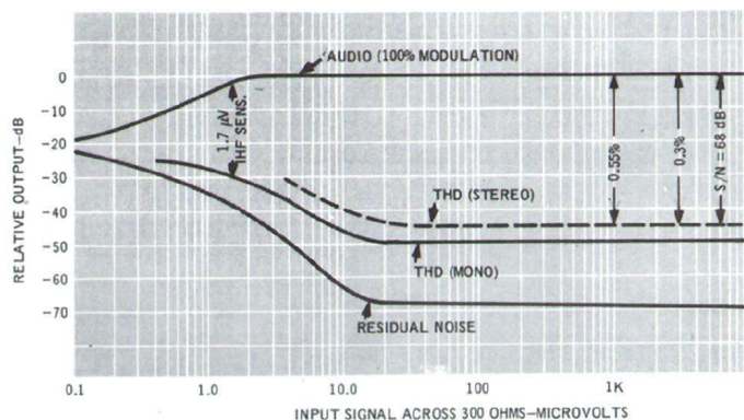
Fig. 3—FM characteristics.
