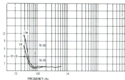
Fig. 4—Low frequency distortion and some SPL measurements.
