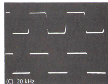
Fig. 2—Oscilloscope traces of PAT-4 square-wave response.
