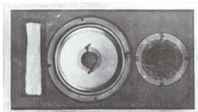
Like the larger A-25 system, the Dynaco A-10 enclosure has a heavily damped port. The tweeter is similar to those in the larger models.
