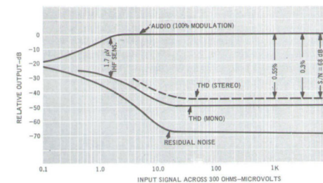
Fig. 3—FM characteristics.
