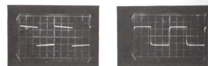
Square-wave response to 50 Hz, left, and to 10 kHz. 15
