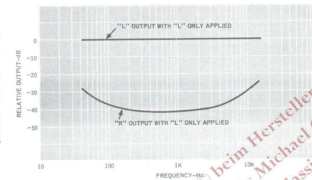
Fig. 4—Stereo FM separation characteristics.
