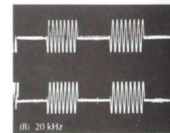
Fig. 3—Tone-burst pattern of PAT-4.
