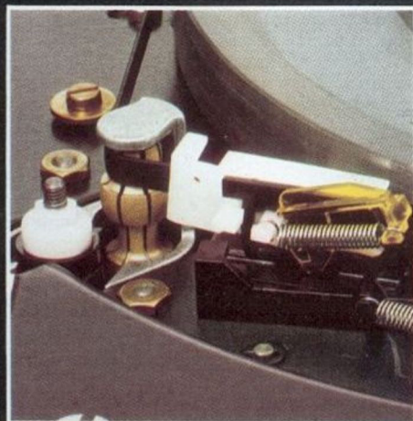
Belt Drive
