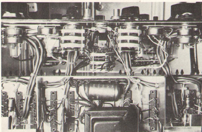
Fig. 11—Underside of electronics chassis.
