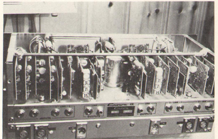
Fig. 12—Back view of complete electronics chassis.
