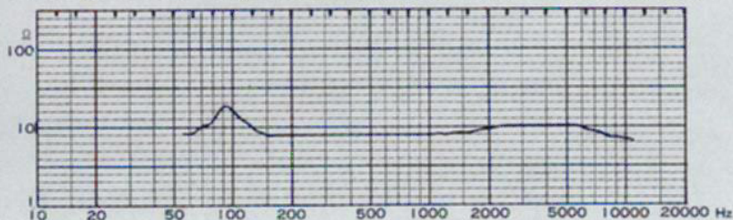
IMPEDANCE CURVE
