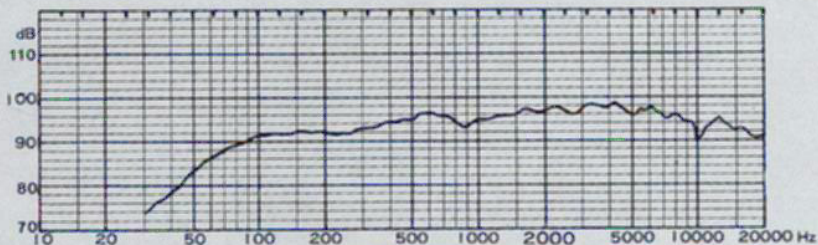
FREQUENCY RESPONSE CURVE
