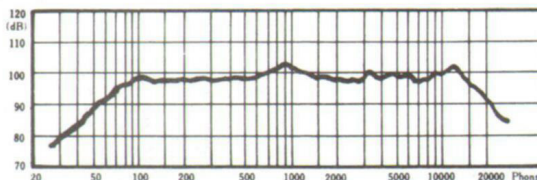
Frequency Response Curve
