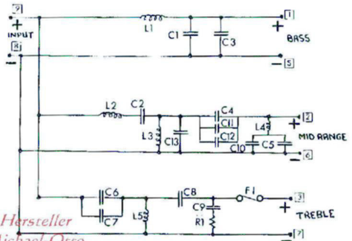
CROSSOVER CIRCUIT DIAGRAM
