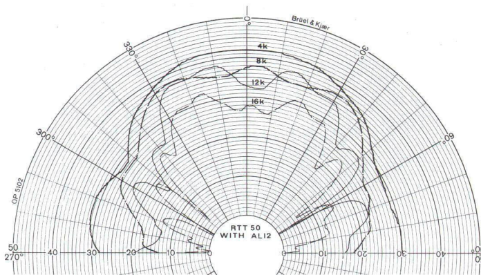
RTT50 WITH AL12 HORIZONTAL POLAR PATTERN
