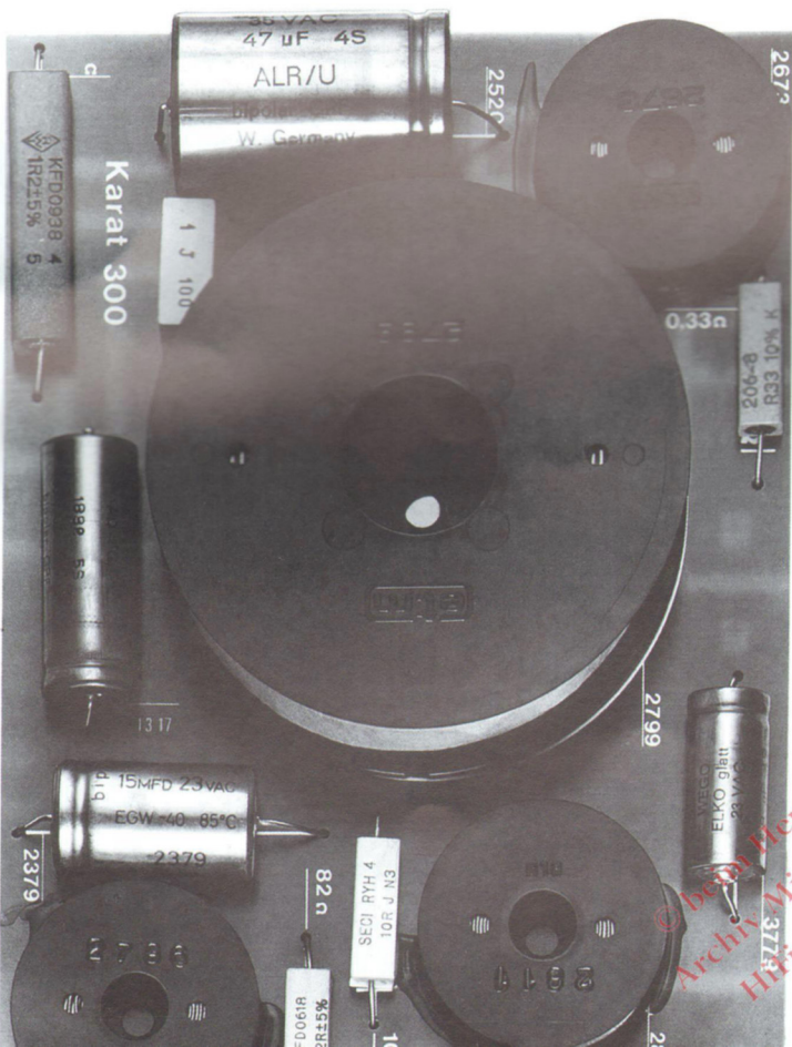
Blicke in die Endmontage: Canton Karat.
