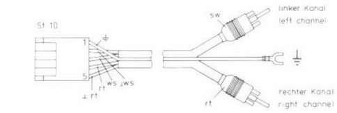
Steckverbindungen pluggable connections
