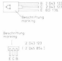
Transistoren transistors
