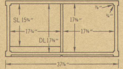
EQUIPMENT CABINET TOP VIEW / INSIDE DIMENSIONS
